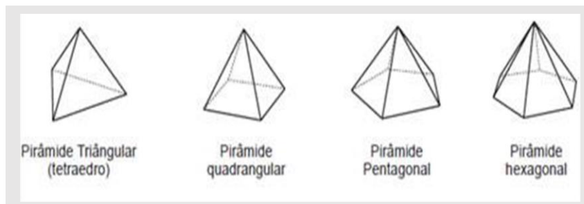
Figura 26 - Pirâmides de base triangular, quadrangular, pentagonal e hexagonal.
