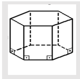
Figura 24 - Prisma hexagonal regular.
