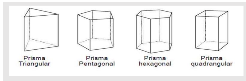
Figura 21 - Prismas de base triangular, pentagonal, hexagonal e quadrangular.
