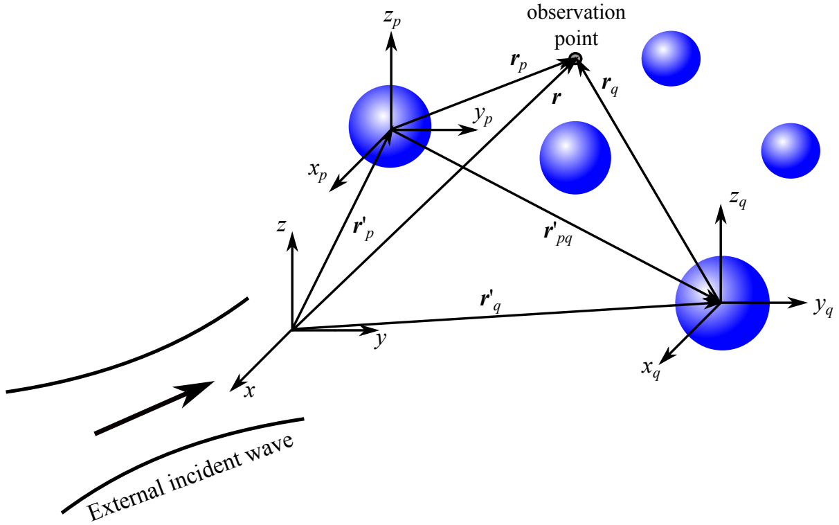
Figure 2.5: Geometric description of the multiple scattering by particles in a suspension. A source particle is located at \mathbf{r}_q and its corresponding scattered wave is probed at \mathbf{r}_p .
