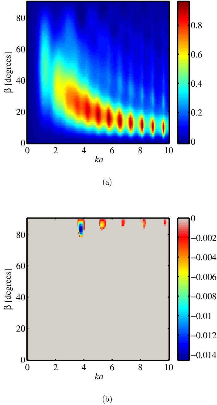
Figure 4.6: Axial radiation force function Y_z for the silicon oil sphere due to the first-order Bessel beam. The function Y_z is normalized to 0.4201. (a) The sphere location has a offset of kx_0 = 1.6 along the x -axis. (b) The islands of attractive radiation force in the off-axial configuration.
