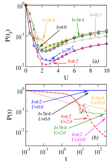
Fig. 4. (a) Purity function computed ( P(t_f) ) after 100 time units versus interaction ( U ) for distinct applied electric pulses. The degree of entanglement displays a non-monotonic dependence on U and is greater for electric pulses which promote higher velocities of the unbound branch. (b) For an intermediary interaction strength the time evolution of quantum purity function indicates that the wave-packet develops a continuously increasing degree of quantum entanglement when the electric pulse promote higher velocity of the unbound branch.
