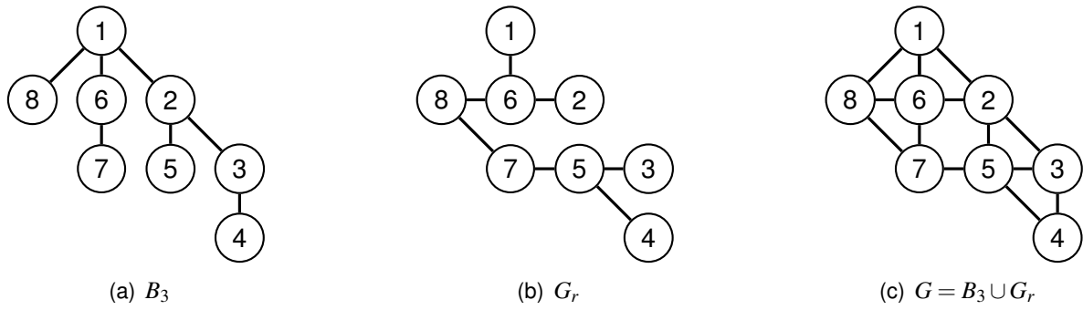
Figure 2.2: Building a synthetic instance.
