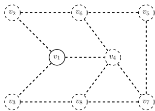
Figure 2.4: Input graph
