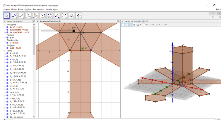
Figura 21: Prisma reto de base hexagonal regular planificado
