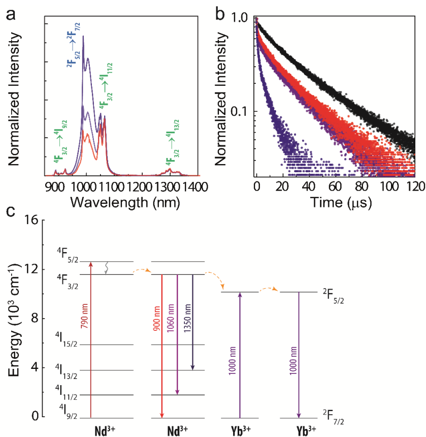
Figure 5.3 - (a) The room temperature emission spectra of \text{Nd@Yb LaF}_3 (red), \text{Yb@Nd LaF}_3 (purple) and \text{Nd:Yb LaF}_3 (blue) NPs under 808 nm laser excitation (97 mW). The transitions ascribed to \text{Nd}^{3+} and \text{Yb}^{3+} are identified in green and blue, respectively. Spectra are normalized to their intensity at 1350 nm. (b) Fluorescence lifetime of the {}^4\text{F}_{3/2} \text{Nd}^{3+} emitting level of \text{Nd@Yb} (red), \text{Yb@Nd} (purple) and \text{Nd:Yb LaF}_3 (blue) NPs. The decay curve obtained for \text{Nd LaF}_3 NPs (black) is included for comparison. (c) Simplified energy scheme of the \text{Nd}^{3+} and \text{Yb}^{3+} emitting centers representing excitation and radiative decays (full lines), non-radiative decays (curved line) and possible ion-ion energy transfer paths (dashed lines).
