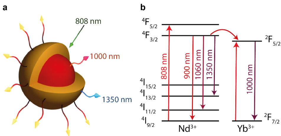
Figure 4.7 - (a) Schematic representation of the proposed Yb@Nd* LaF 3 NPs. (b) Simplified energy scheme of the Nd 3+ and Yb 3+ emitting centers representing excitation and radiative decays (full lines) and possible ion-ion energy transfer paths (curved lines).
