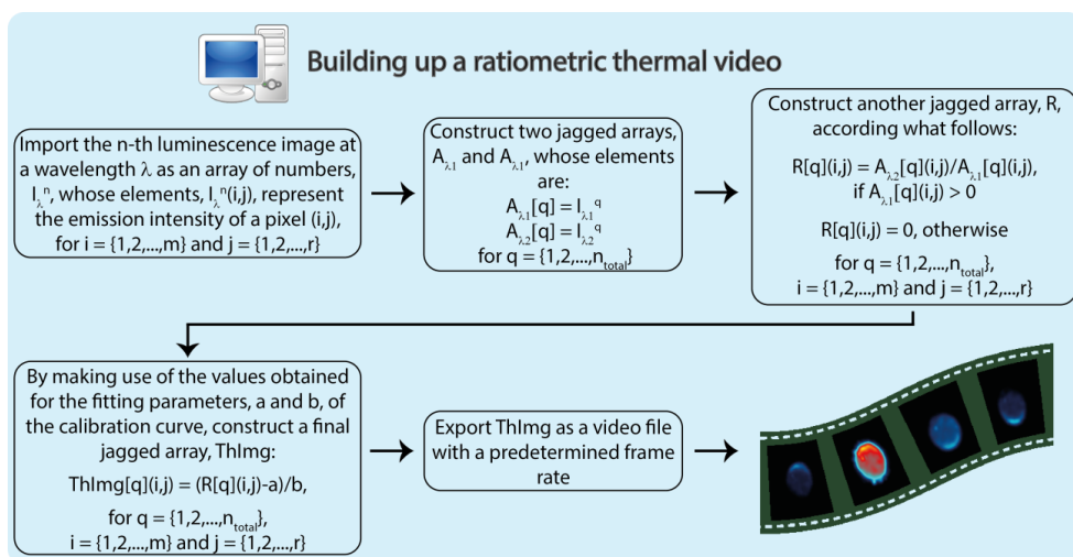
Figure 3.9 - Flowchart followed by the home-made software to build up a thermal image from fluorescence images. m \times r stands for the resolution of the fluorescence images, while n_{\text{total}} corresponds to the total number of fluorescence images obtained at each wavelength range.
